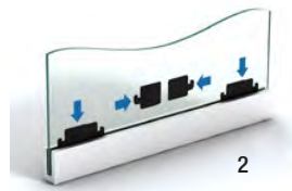
Install TAPER-LOC® Tapers with CRL's TLK12 Installation/Removal Tool to lock the glass securely in place.
