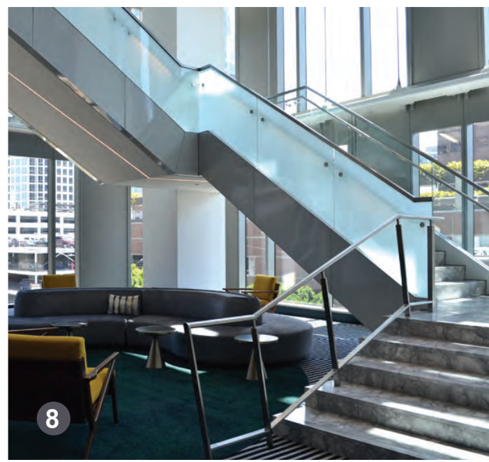
7) GRS Glass Railing System Bridge with Cap Rails 8) GRS Stainless Steel Glass Railing System with HRS Hand Rails and Custom-Fabricated Stainless Steel Post System
